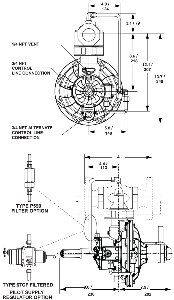
Figure 8. Types 299H and 299HR Dimensions
