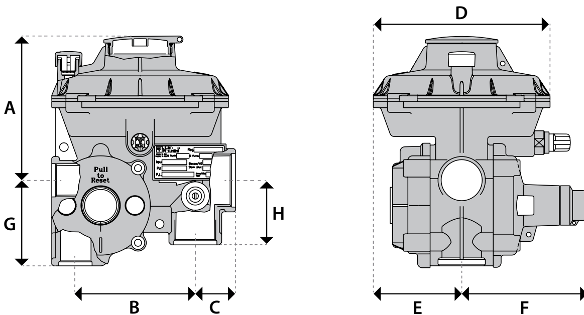
Figure 8 FE515 STD Dimensions
