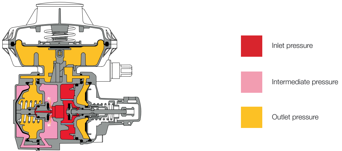
Figure 4 FE515 with slam shut
