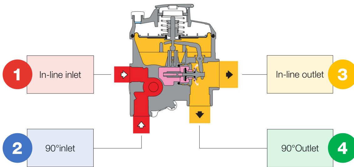
Figure 7 Fittings
